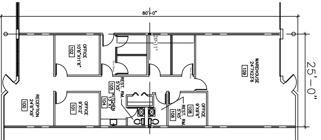
FLOOR PLAN SUITE "F" 3/32" = 1'-0"
